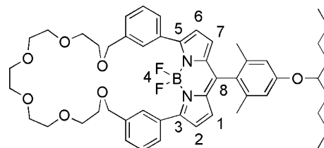
Figure 1. Chemical structure of boron–dipyrrromethene fluoroionophore 1 .
